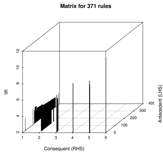
Figure 6: Matrix-based visualization with 3D bars.
