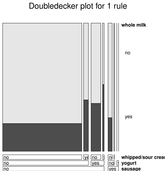
Figure 13: Double decker plot for a the rule sausage,yogurt,whipped/sour cream => whole milk.
